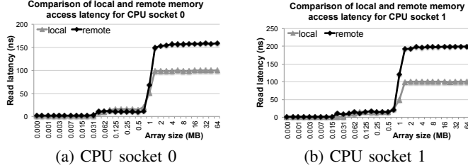
Fig. 2: The comparison of local and remote memory read latency for various memory sizes, with a stride size of 64 bytes. The results are reported in nanoseconds per load.
