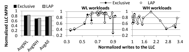
Figure 18: LLC MPKI of different policies normalized to the non-inclusive policy.
