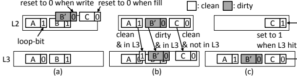
Figure 10: The update of loop-bits during (a) L2 insertions, L2 modifications, (b) L2 evictions, and (c) L3 hits.
