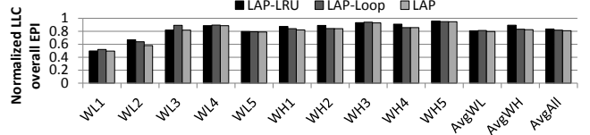
Figure 19: LLC overall EPI of LAP-LRU, LAP-Loop, and LAP normalized to the non-inclusive LLC.
