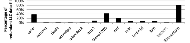
Figure 6: Distribution of redundant LLC data-fill.
