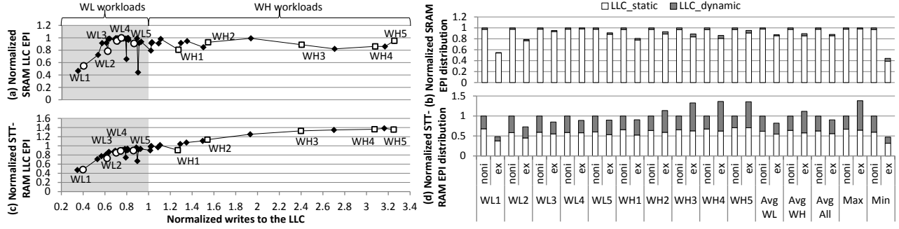
Figure 12: EPI of the exclusive policy (ex) normalized to the non-inclusive policy (noni) in the (a) SRAM and (c) STT-RAM LLC. The energy breakdown of sampled workloads are shown in (b) and (d). WL/WH workloads: fewer/more writes in the exclusive policy.
