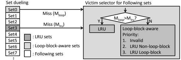
Figure 9: Loop-block-aware replacement policy.
