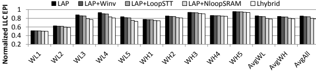
Figure 25: LLC EPI of different data placement policies in the hybrid LLC, normalized to the non-inclusive policy. Winv: invalidating STT-RAM block when write-hit. LoopSTT: storing loop-blocks in STT-RAM. NloopSRAM: storing non-loop-blocks in SRAM.
