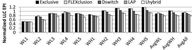
Figure 24: Hybrid LLC EPI normalized to non-inclusive policy.
