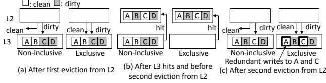
Figure 3: Illustration of redundant clean data insertion.
