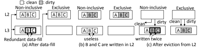
Figure 5: Illustration of redundant LLC data-fill.
