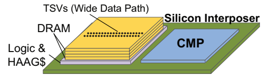
Figure 1: The target system design for integrating the HAAG$: a hybrid 3D DRAM stack and a chip multiprocessor are co-located on a silicon interposer.
