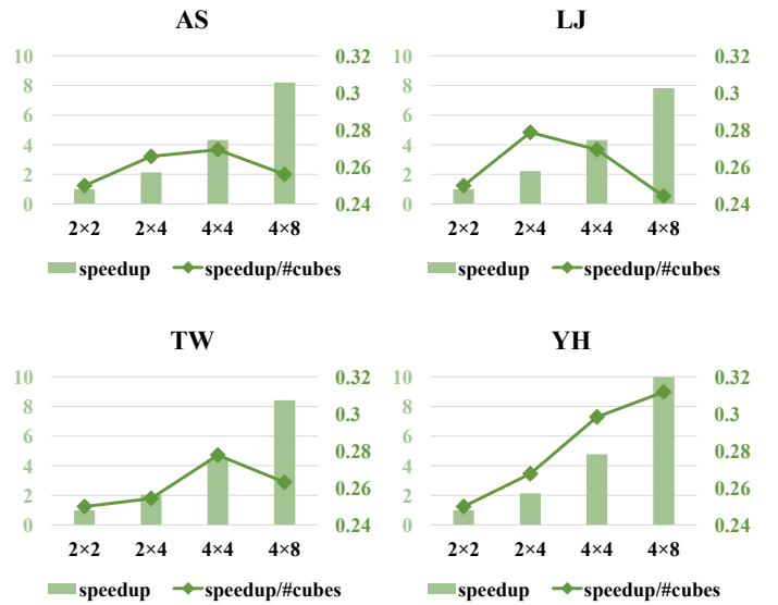
Fig. 17. Performance on different array sizes.
