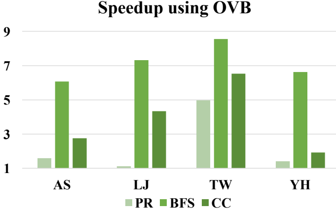
Fig. 9. Speedup using On-chip Vertex Buffer.
